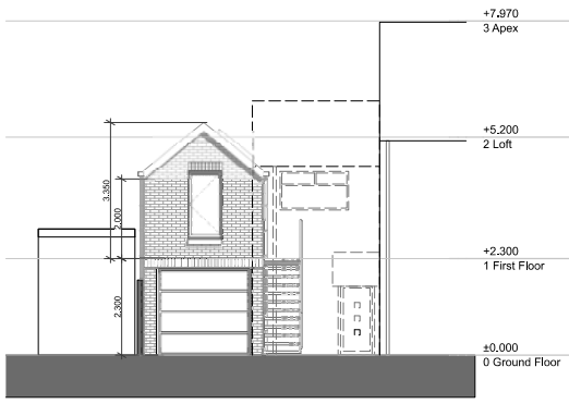
E-05 E-05 Proposed East Elevation 1:100
