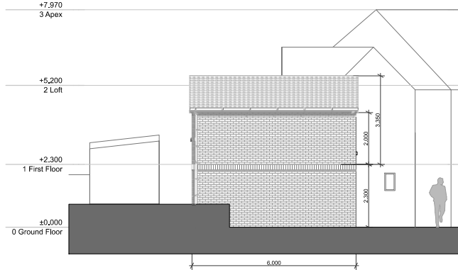
E-08 E-08 Proposed South Elevation 1:100
