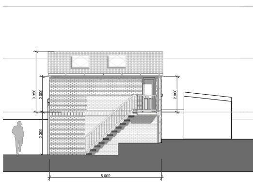
E-07 E-07 Proposed North Elevation 1:100
