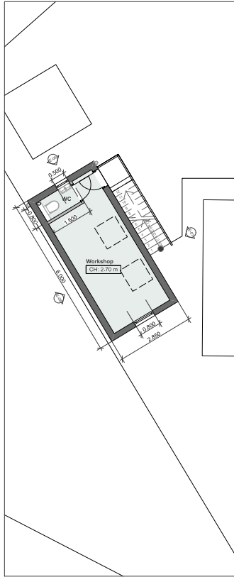
PL-02 PL-02 First Floor Plan 1:100
