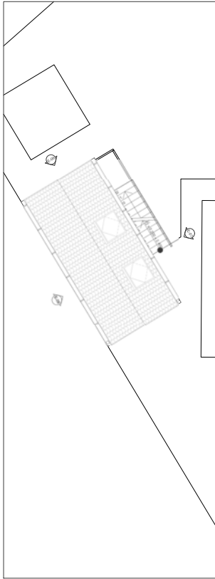
4 PL-03 Roof Plan 1:100
