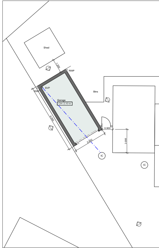
PL-01 PL-01 Ground Floor Plan 1:100
