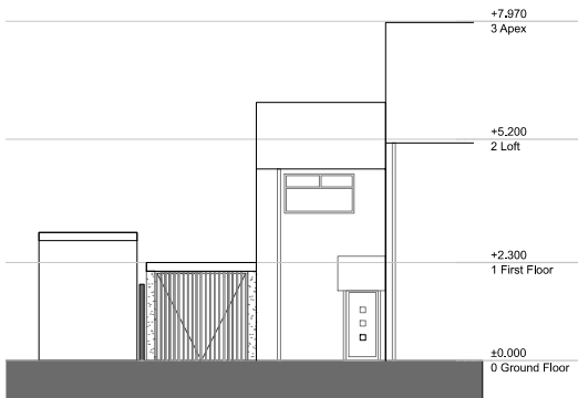
E-01 Existing East Elevation 1:100
