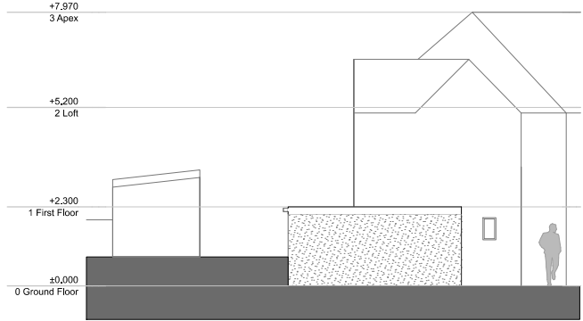
E-04 Existing South Elevation 1:100
