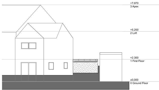
E-02 Existing West Elevation 1:100
