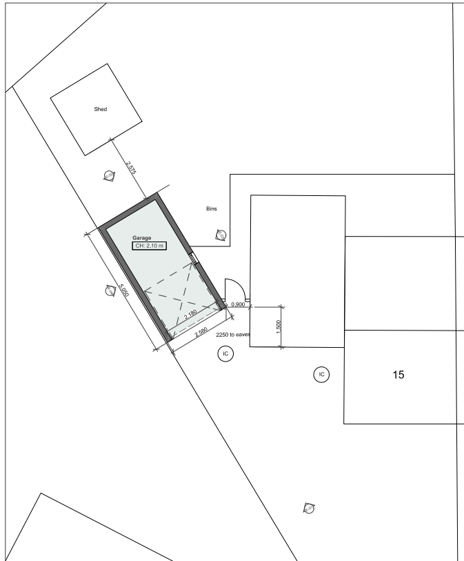
PL-01 Ground Floor Plan
