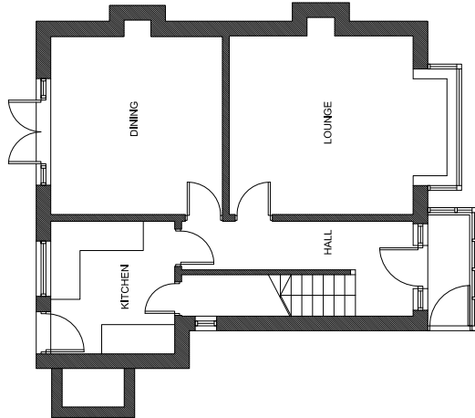
EXISTING GROUND FLOOR PLAN SCALE 1:100
