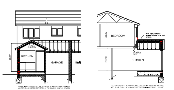
PROPOSED SECTION A-A
