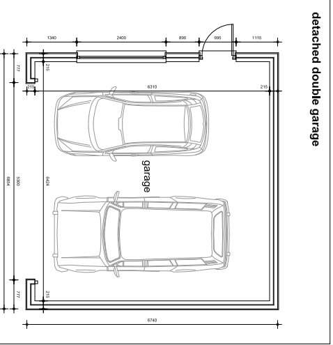
detached double garage floor plan Scale: 1:50
