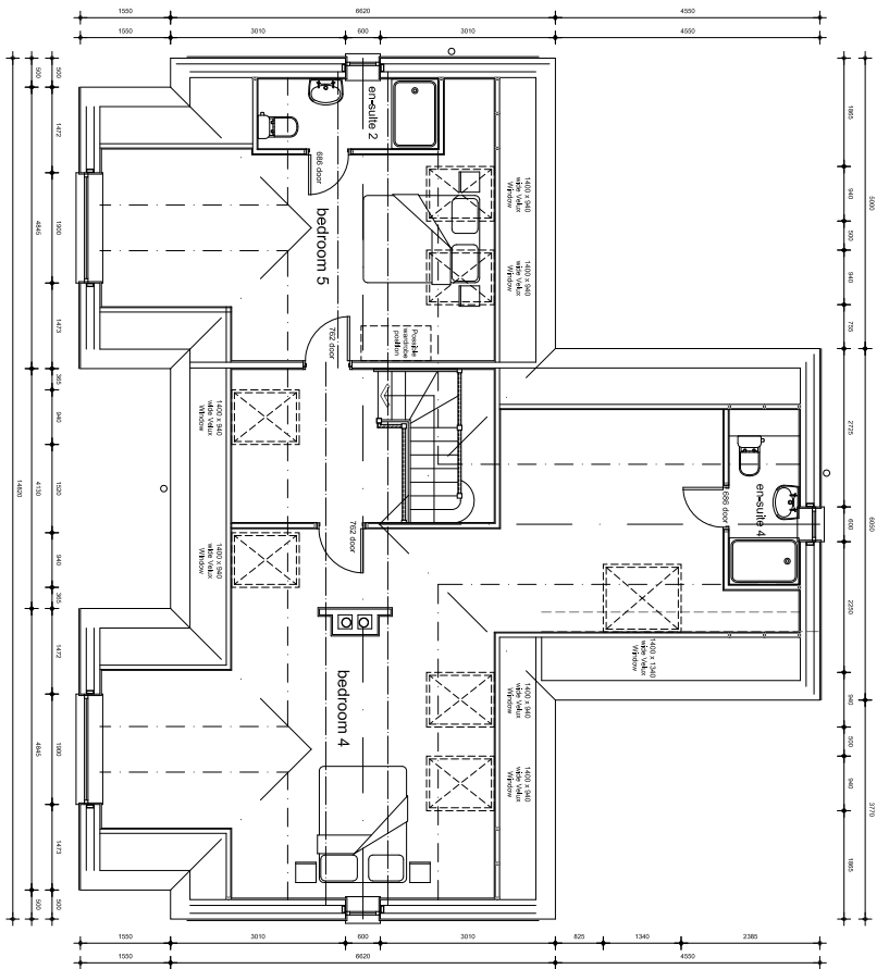
second floor plan Scale: 1/50
