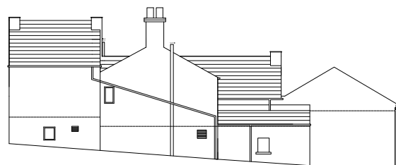
WESTERN FACING ELEVATION
