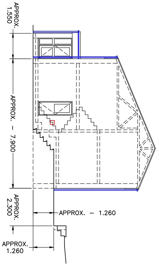
EXISTING SOUTH WEST SIDE ELEVATION
