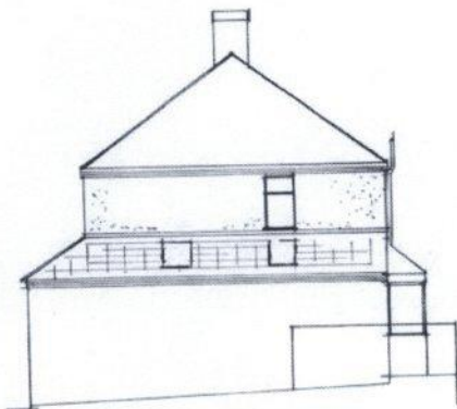
PROPOSED SIDE
