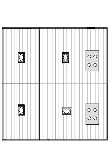
R1 Roof 1:50
