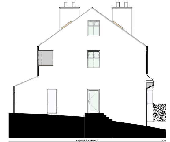
Proposed Side Elevation 1:50
