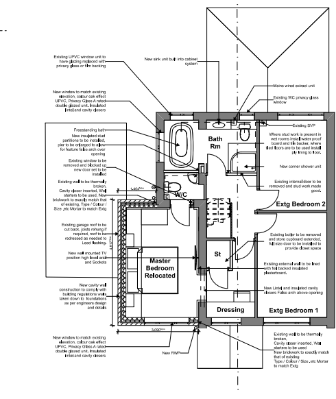
Proposed First Floor 1:50
