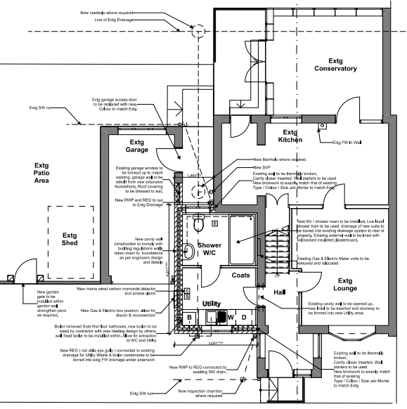
Proposed Ground Floor 1:50
