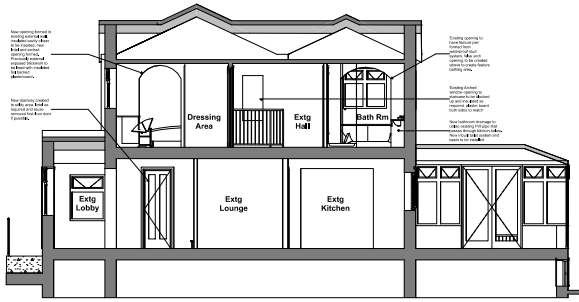
Proposed Building Section 1:50
