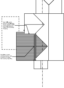
Proposed Roof 1:100
