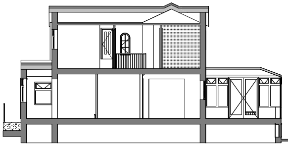
Building Section 1:50
