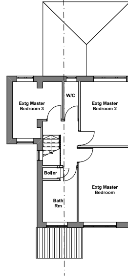
First Floor 1:50
