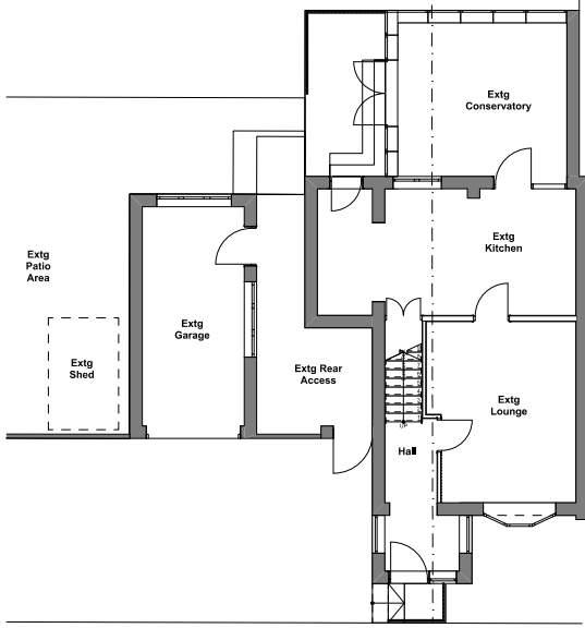
Ground Floor 1:50
