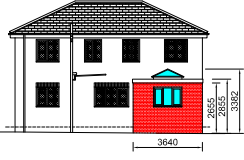
Proposed Rear Elevation
