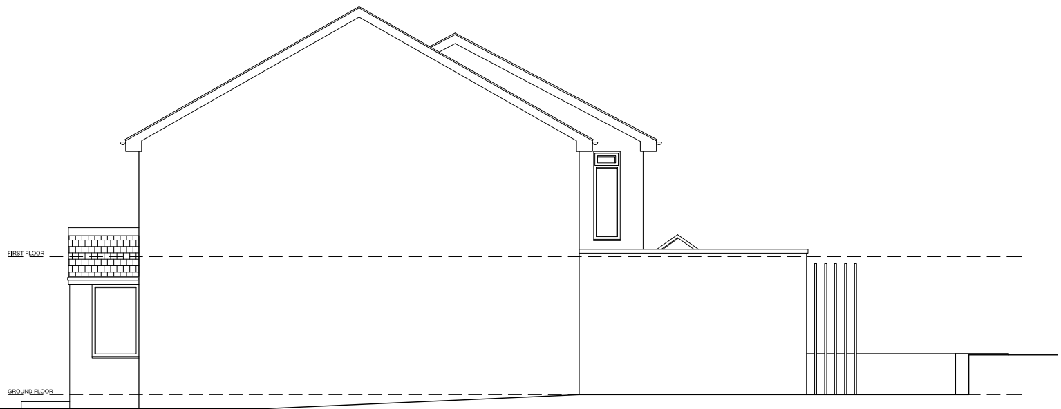
PROPOSED (RIGHT) SIDE ELEVATION SCALE 1:50
