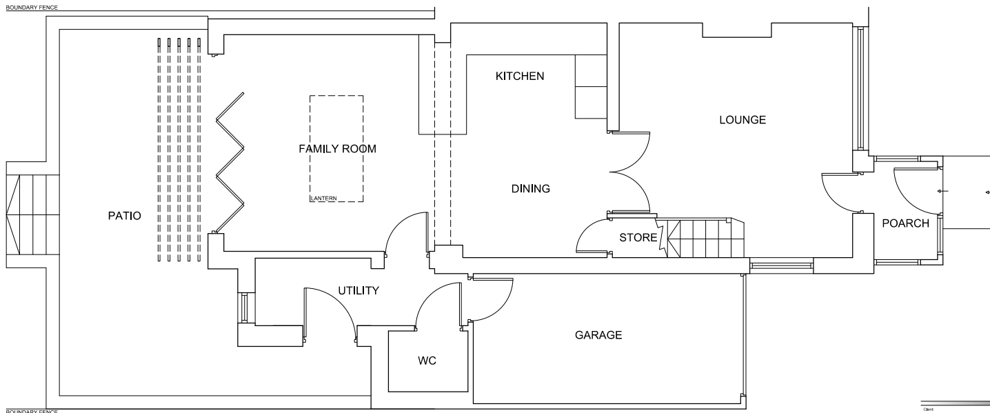
PROPOSED GROUND FLOOR PLAN SCALE 1:50
