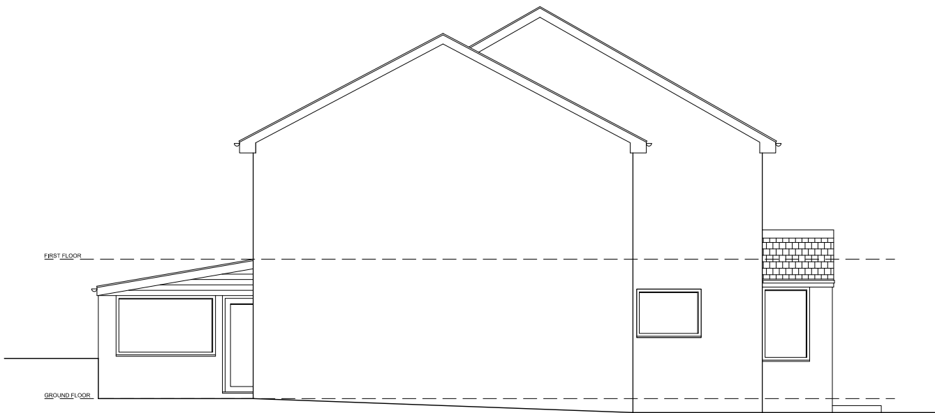
EXISTING (LEFT) SIDE ELEVATION SCALE 1:50
