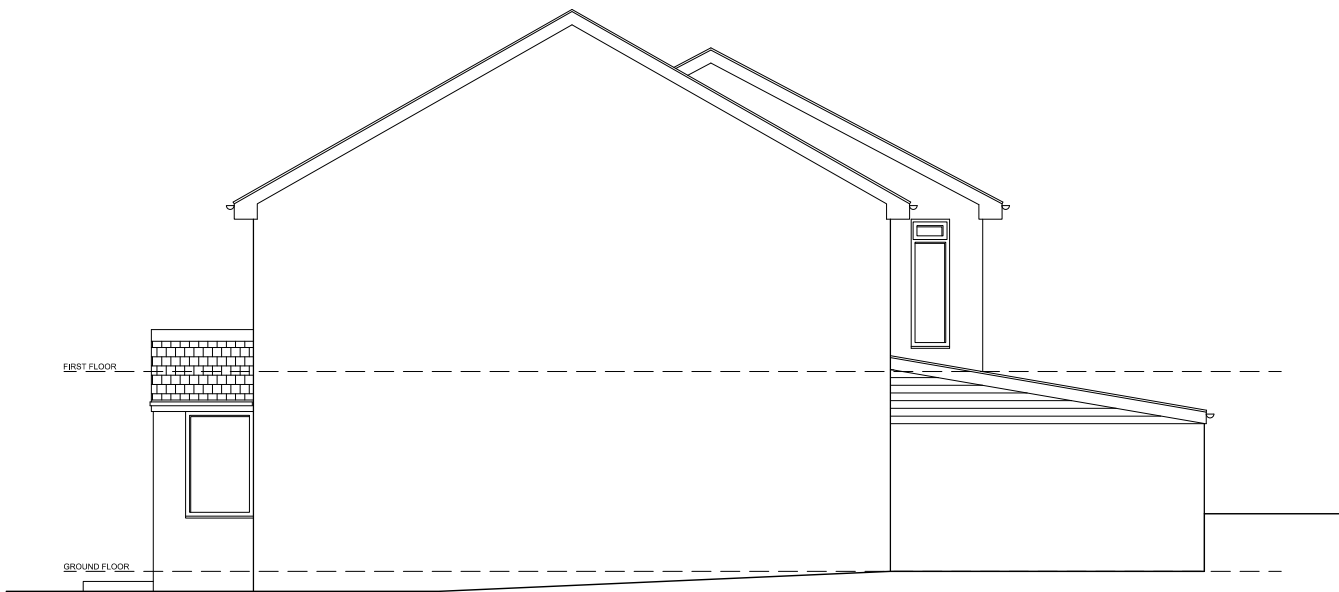
EXISTING (RIGHT) SIDE ELEVATION SCALE 1:50
