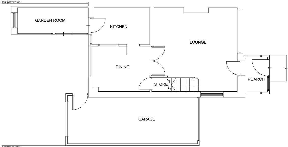
EXISTING GROUND FLOOR PLAN SCALE 1:50
