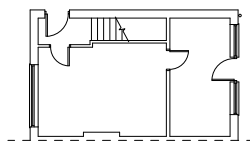
EXISTING FLOOR PLANS SCALE 1:100
