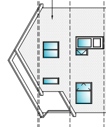
PROPOSED FRONT ELEVATION SCALE 1:100
