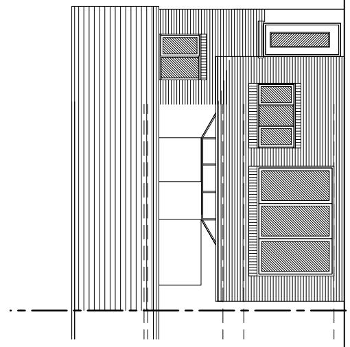
EAST ELEVATION 1:50
