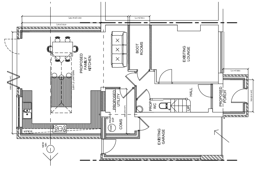
GROUND FLOOR PLAN 1:50
