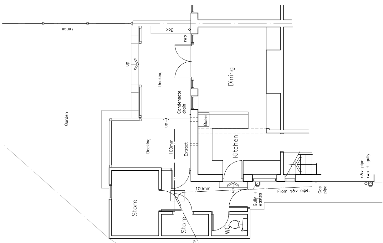
GROUND (1:50)
