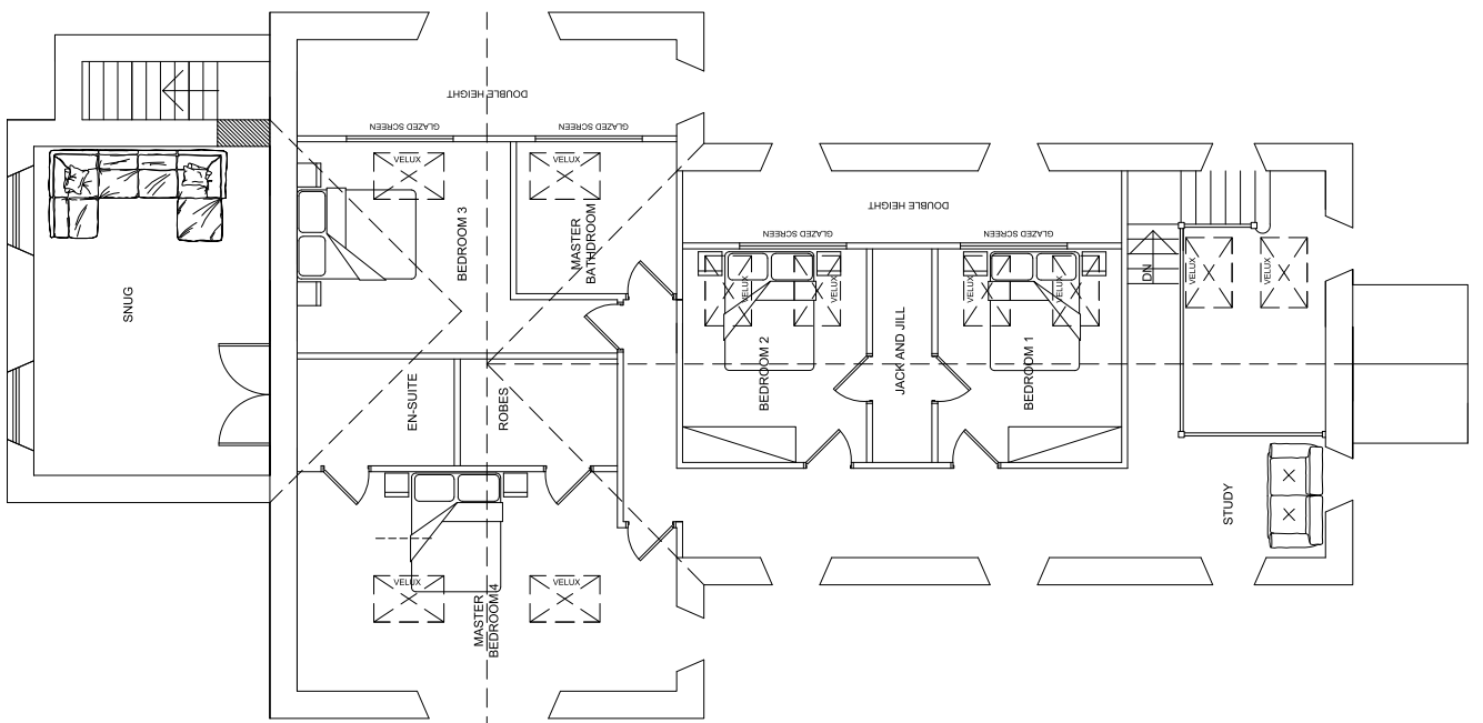
FIRST-FLOOR-PLAN-1:50
