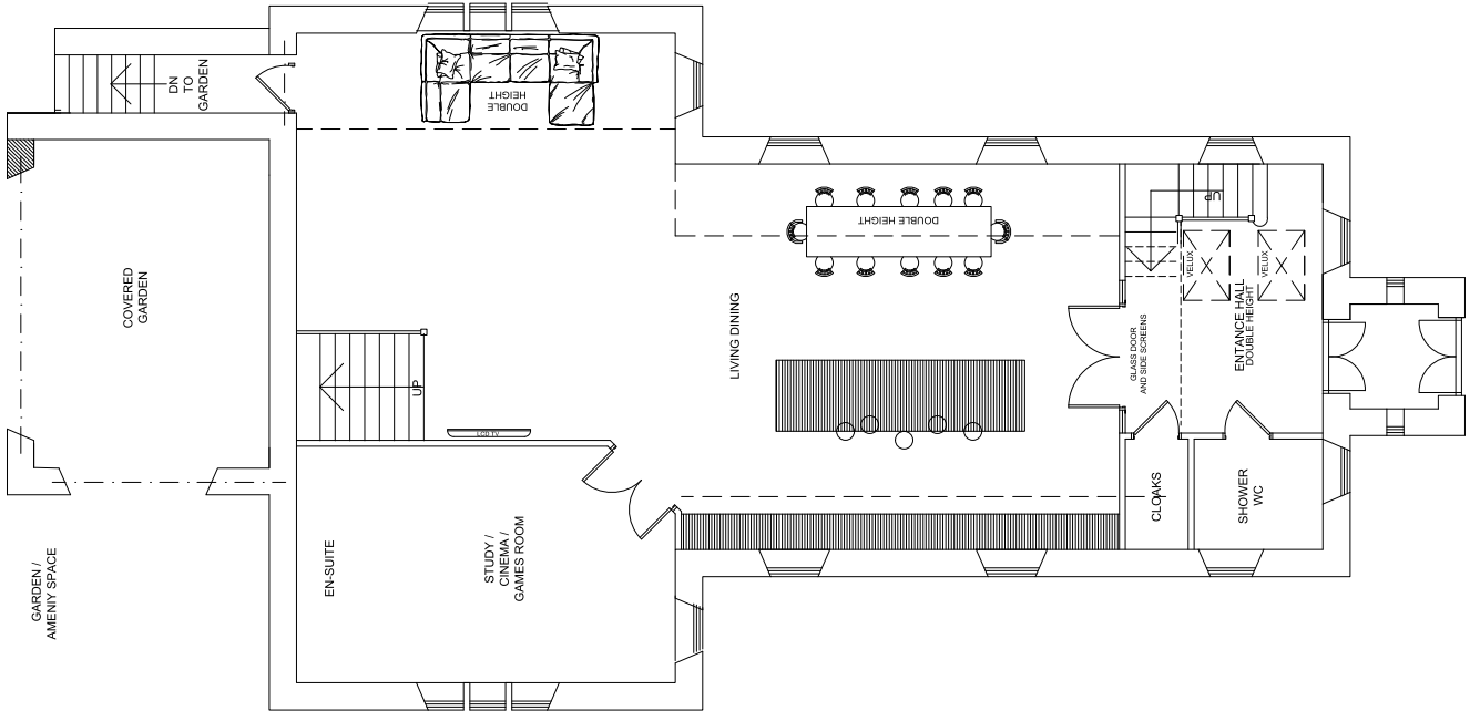
GROUND FLOOR PLAN 1:50
