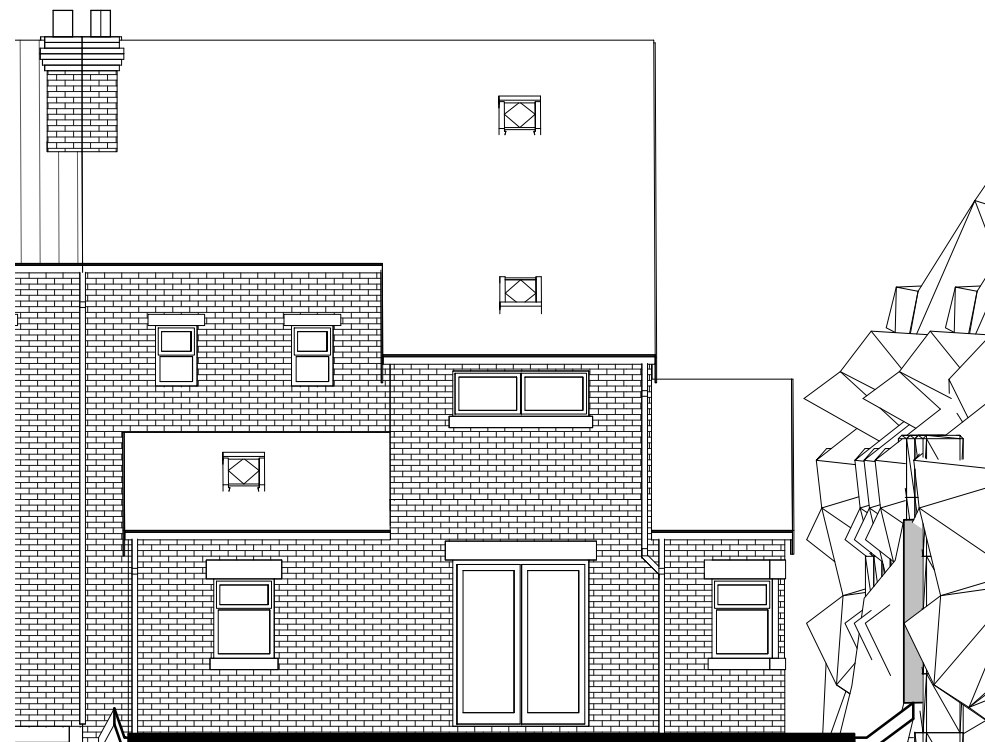
3 Rear Elevation 1 : 100
