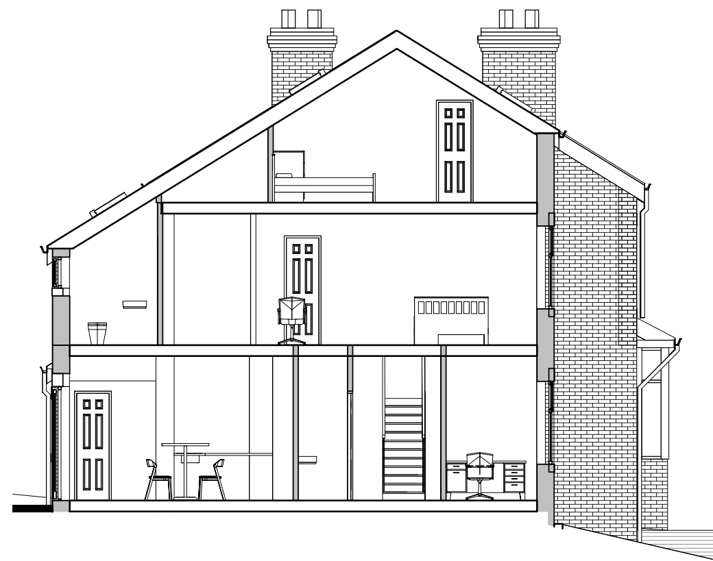
4 Proposed Section 1 : 100
